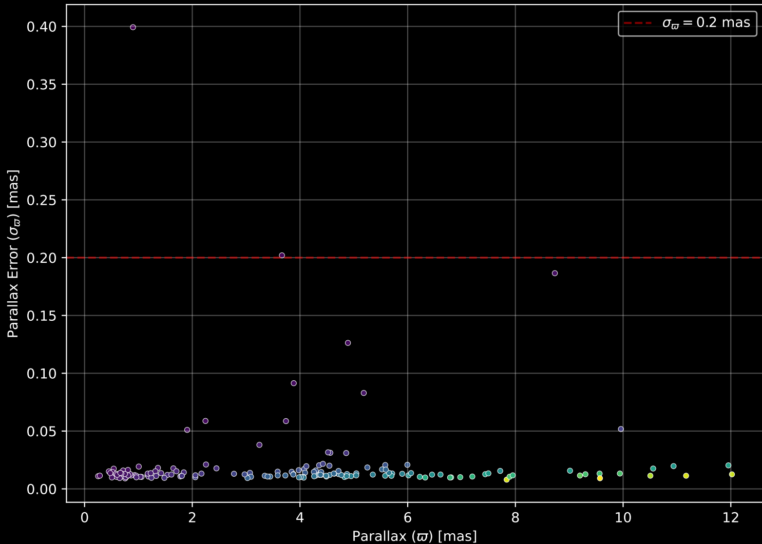
APOGEE DR17 Field: [CVZTILE_096+22_btx] Parallax Quality (n= 164)
