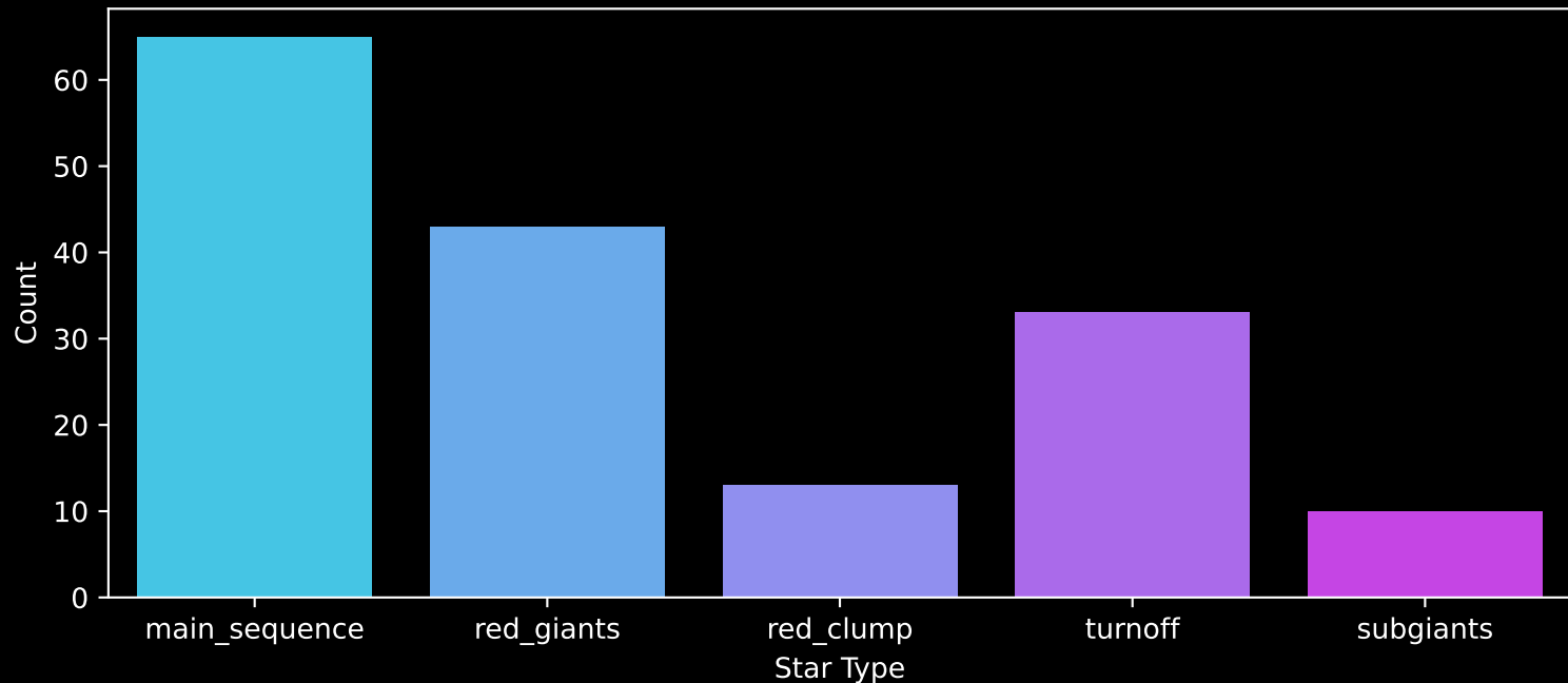
APOGEE DR17 Field: [CVZTILE_096+22_btx] Count plot of Star Type
